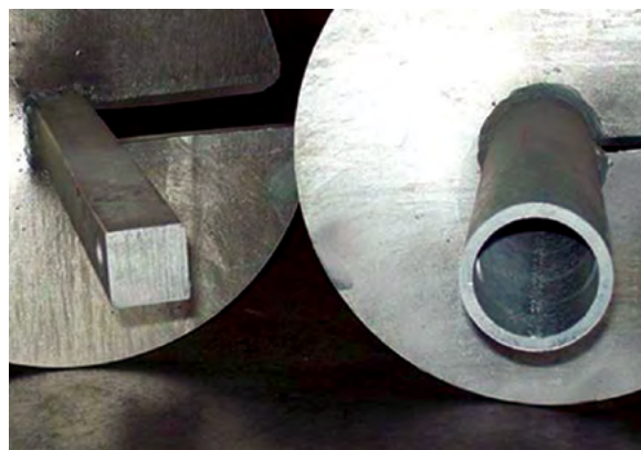
Figure 2.3.2.2.a Section comparison between 2.875" diameter, 0.276" wall round shaft and 1.5" square shaft
