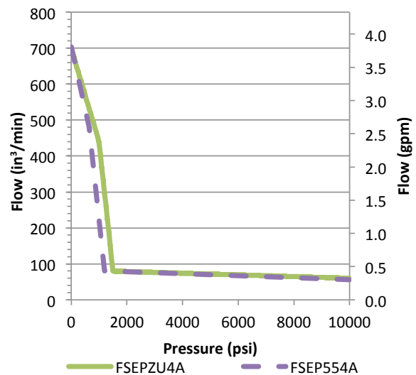
Figure 3.8.2.2.a FSI Electric Powered Hydraulic Pump Curves
