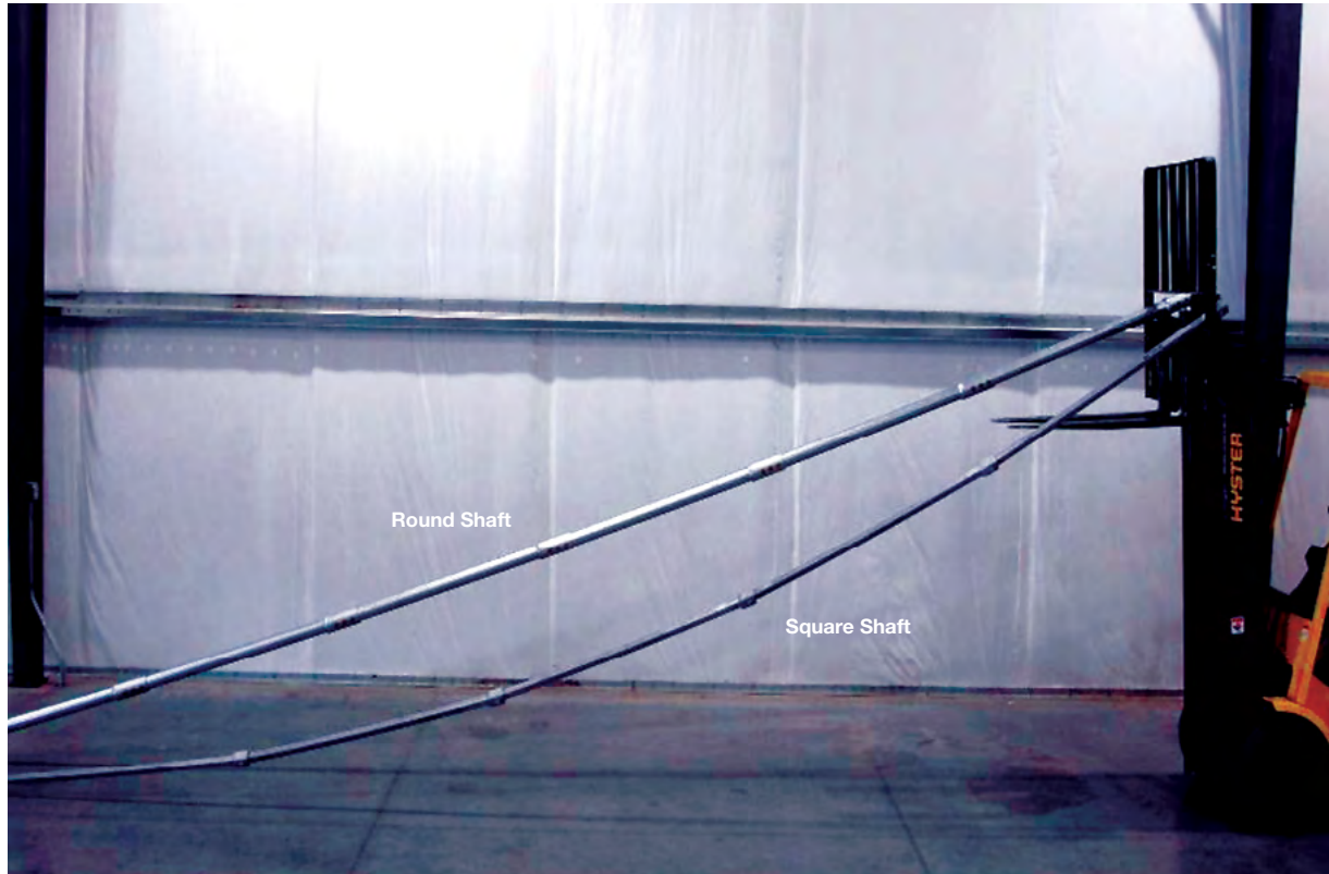
Figure 2.3.2.1.j Coupler Rigidity Comparison: FSI round shaft external welded coupler vs. typical upset coupler for square shaft
