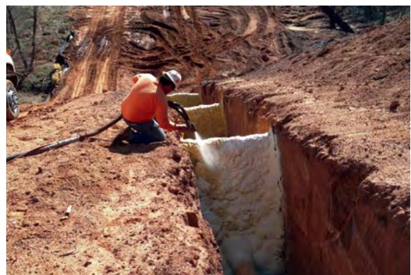
Figure 5.2.e Placement of polyurethane foam trench breaks
