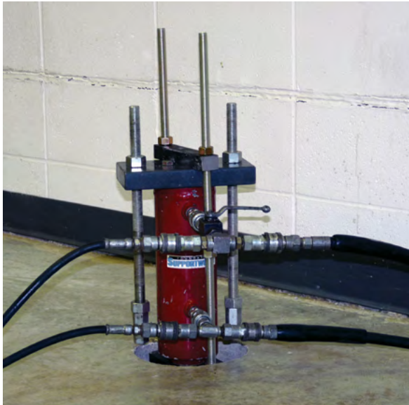
Figure 3.12.q Hydraulic connections at lift cylinder
