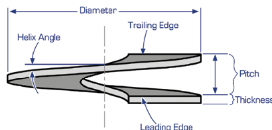
Figure 2.3.1.b Helix Plate Geometry
