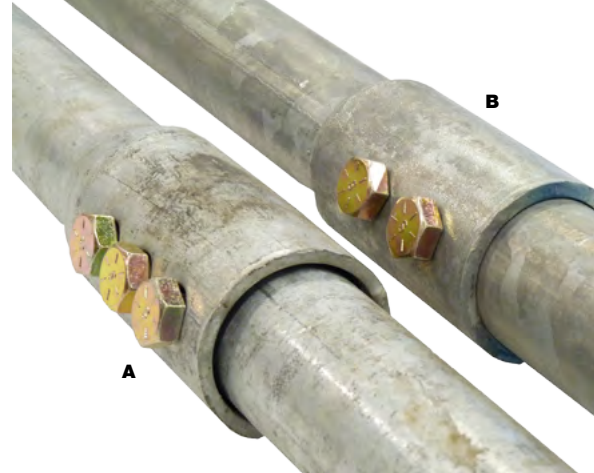
Figure 2.3.2.1.d Coupler tolerances; (A) Competitor upset coupler, (B) FSI external welded coupler
