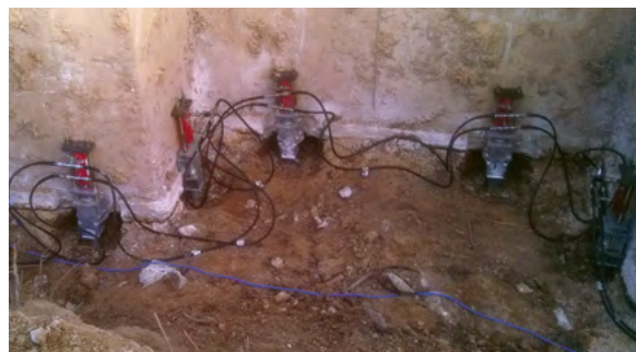
Figure 3.10.p2 Hydraulic system connected to provide uniform application of load
