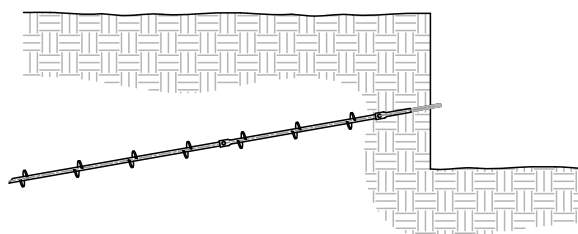
Step 2 - Install top row of soil nails
