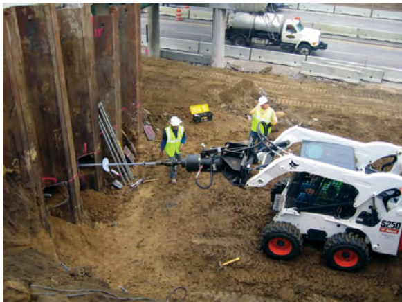
Sheet pile wall stabilization with helical tiebacks
