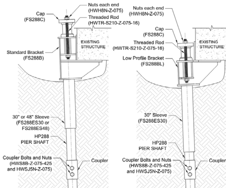
FIGURE 1—HP288 RETROFIT BRACKET AND SHAFT ASSEMBLIES
