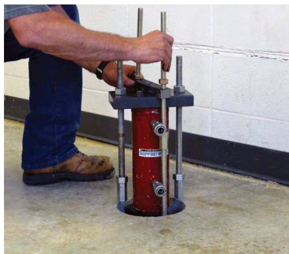
Figure 3.12.p Lift plate assembly coupled to threaded rods of slab pier bracket
