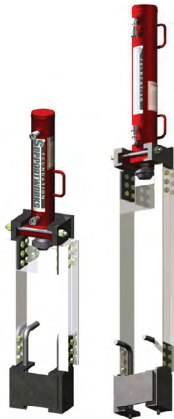
Figure 3.8.5.a Crawl space and standard drive stand assemblies for the PP288 push pier system
