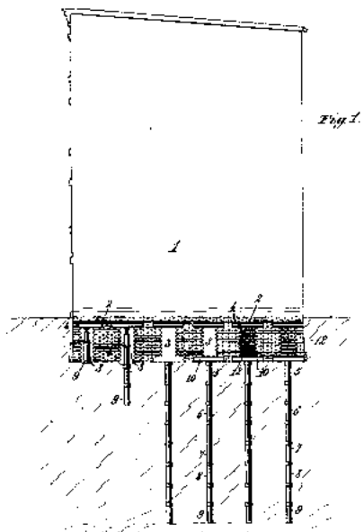
Figure 3.1.a Breuchard patented system (1896)
