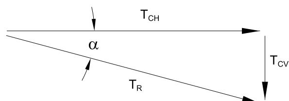
Figure 2.8.1.b Vector mechanics of tieback forces
