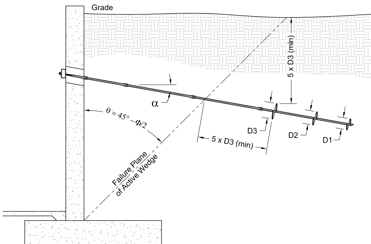
Figure 2.8.1.a Helical tieback design considerations
