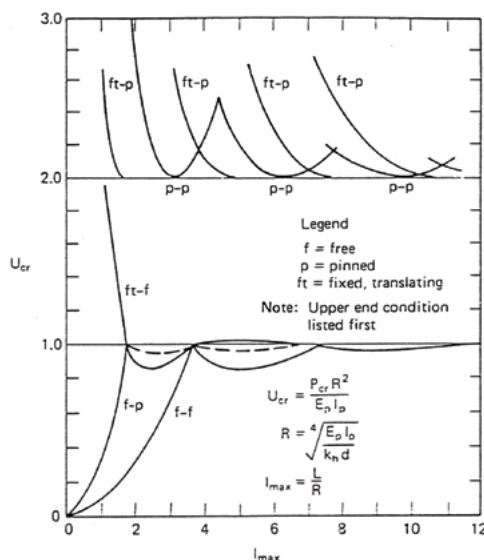
Figure 2D.1 Buckling load (load coefficient) vs. length (depth coefficient) for k_h = constant (Davisson 1963)
