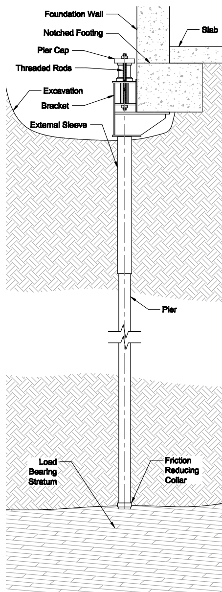
Figure 3.2.b FSI PP288 push pier system with an under-footing bracket
